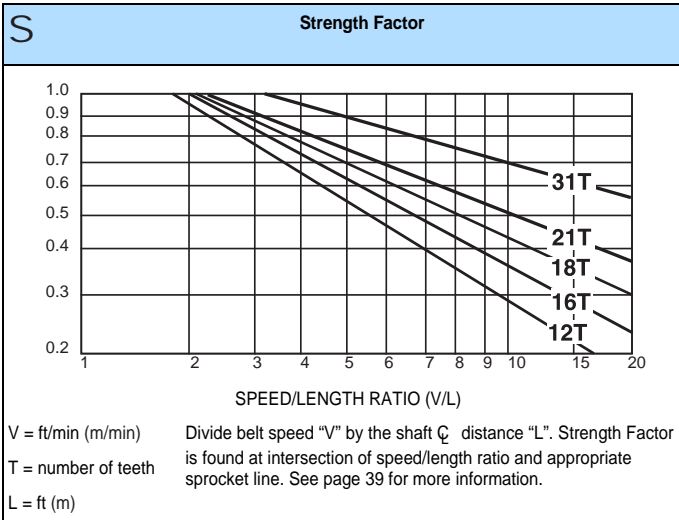
Plastic Sprocket Data a
