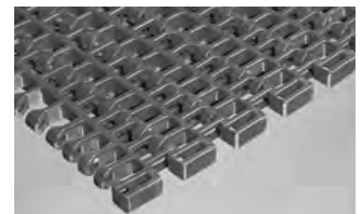
SERIES 2600 (2.5) • Hinge- driven • Open hinge • Sideflexing • 2.00 in. (50.8 mm) pitch
