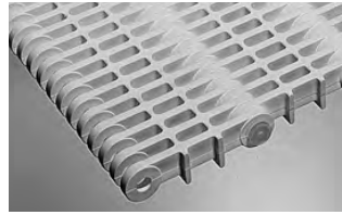
SERIES 200 • Hinge-driven • Closed hinge • 2.00 in. (50.8 mm) pitch • Non flush edge
