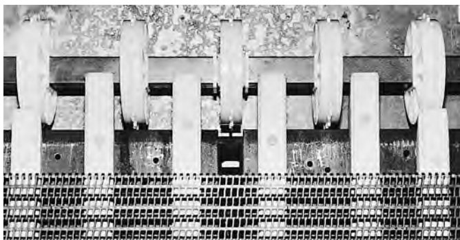
Fig. 3-10 Anti-sag configuration
