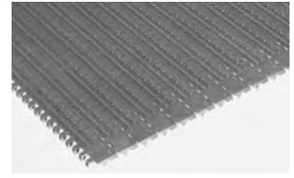
SERIES 1600 • Center-driven • Open hinge • 1.00 in. (25.4 mm) pitch
