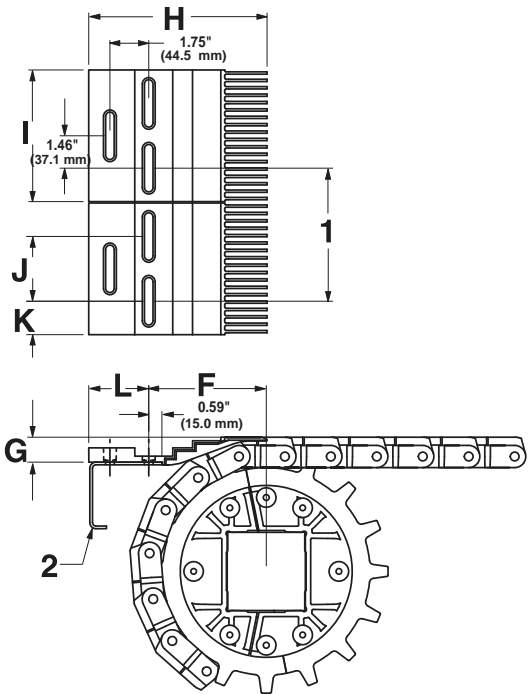
Dimensional Requirements for Self-Clearing Finger Transfer Plate Installations a
