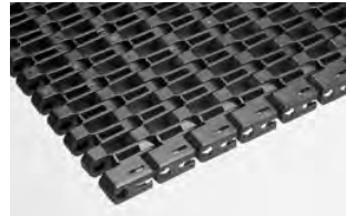
SERIES 1700 • Center/Hinge- driven • Closed hinge • 1.50 in. (38.1 mm) pitch
