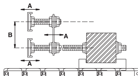
Fig. 2-23 Dual blade pusher bar assembly
