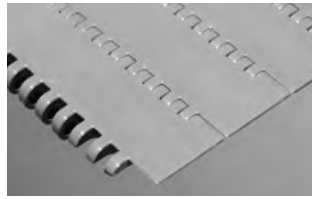
SERIES 900 FLAT TOP • Center-driven • Closed hinge • 1.07 in. (27.2 mm) pitch • Available widths: 4.7 in. (119 mm) and 6.0 in. (152 mm)
