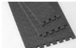
SERIES 1400 FLAT TOP • Center/hinge driven • Closed hinge • 1.00 in. (25.4 mm) pitch • Available widths: 3.25 in. (83 mm), 4.5 in. (114 mm), 6.0 in. (152 mm) and 7.5 in. (191 mm)
