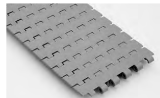
SERIES 1400 6" FLAT TOP WITH SELF-CLEARING EDGE • Center/hinge driven • Closed hinge • 1.00 in. (25.4 mm) pitch • Available width: 6.0 in. (152 mm)
