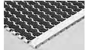
SERIES 1400 OVAL • Center/Hinge-driven • Closed hinge • 1.00 in. (25.4 mm) pitch
