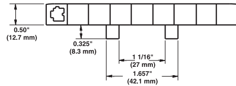
Series 1400 Flat Top Mold to Width
