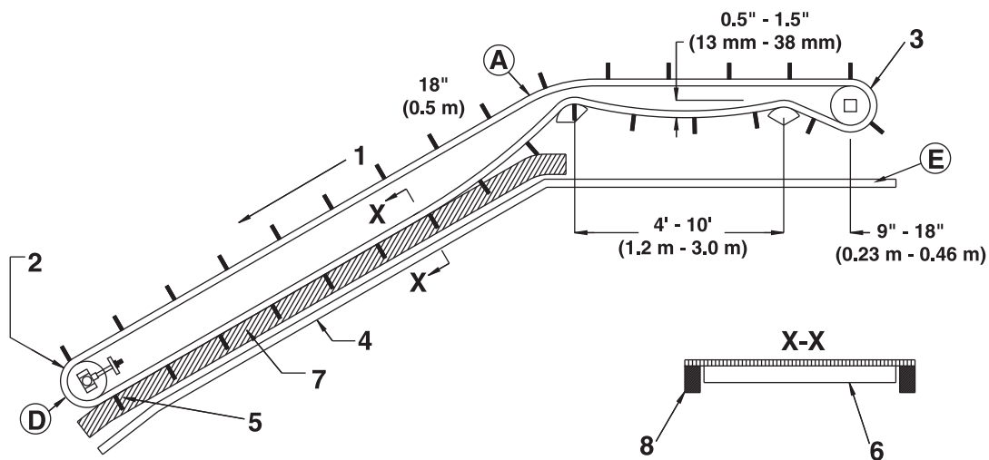
Fig. 3-18 Incline conveyor
