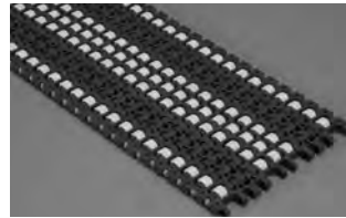
SERIES 1000 INSERT ROLLER TOP • Center/Hinge driven • Closed hinge • 0.60 in. (15.2 mm) pitch • Available width: 6 in. (152 mm)
