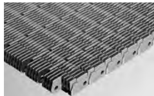
SERIES 1900 • Center/Hinge- driven • Closed hinge • 2.07 in. (52.6 mm) pitch
