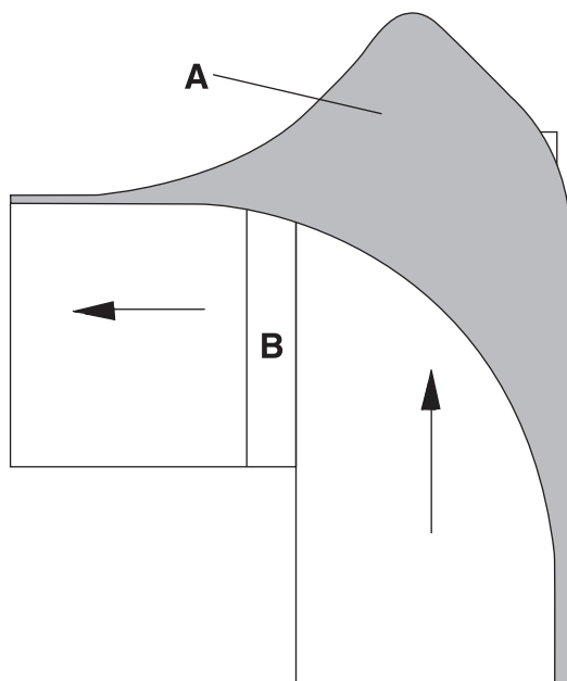
Fig. 3-29 Conventional full radius guide rail contours
