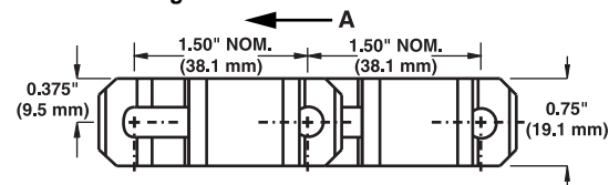
Series 2200 Tab Edge Dimensions
