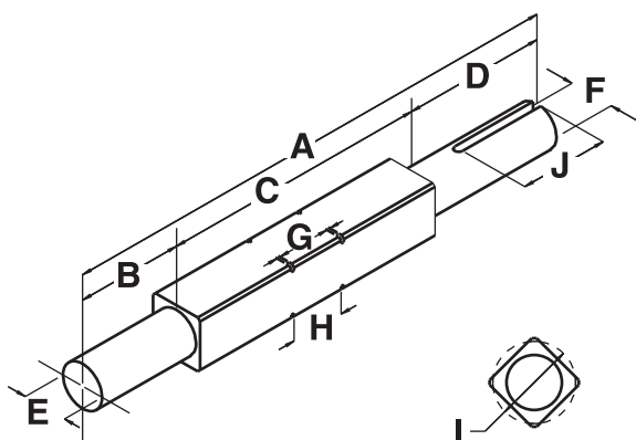
Fig. 2-14 Shaft dimensions
