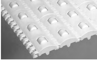
SERIES 800 ROLLER TOP • Center-driven • Open hinge • 2.00 in. (50.8 mm) pitch
