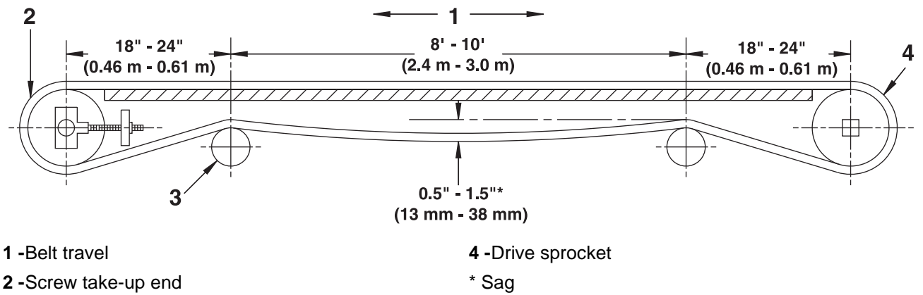
Fig. 3-17 Push-pull bi-directional conveyor
