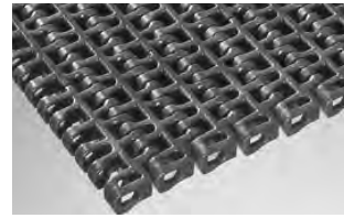
SERIES 1100 • Hinge-driven • Open hinge • 0.60 in. (15.2 mm) pitch
