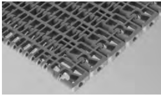
SERIES 900 OPEN FLUSH GRID • Center-driven • Open hinge • 1.07 in. (27.2 mm) pitch
