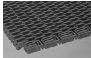
SERIES 800 • Center-driven • Open hinge • 2.00 in. (50.8 mm) pitch
