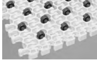
SERIES 2200 INSERT ROLLERS • Hinge-driven • Open hinge • Sideflexing • 1.50 in. (38.1 mm) pitch
