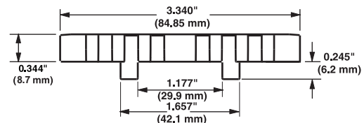
Series 900 Flat Top 85 mm Mold to Width
