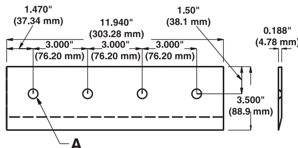
Fig. 2-24 Dead plates
