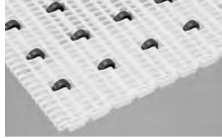
SERIES 900 INSERT ROLLERS • Center-driven • Open hinge • 1.07 in. (27.2 mm) pitch
