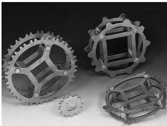
Fig. 2-26 Abrasion resistant (all steel) sprockets
