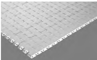
SERIES 1400 EASY RELEASE PLUS • Center/hinge-driven • Closed hinge • 1.00 in. (25.4 mm) pitch
