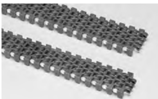
SERIES 1100 FLUSH GRID • Hinge driven • Open hinge • 0.60 in. (15.2 mm) pitch • Available widths: 1.5 in. (38 mm) and 1.8 in. (46 mm)
